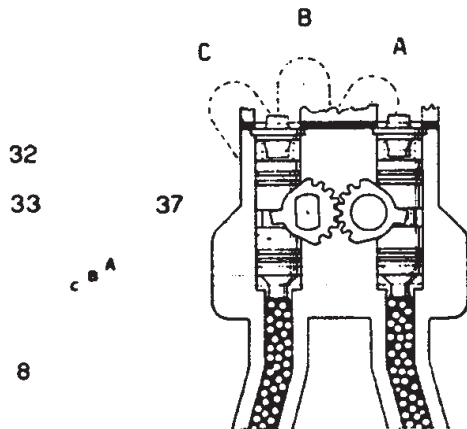
Fig. 17 - STARTING DEVICE.
